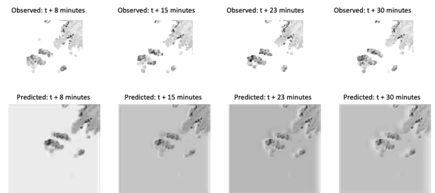
Figure 5. Frame prediction of the second ConvLSTM approach: comparison between real and predicted frames. The observed frames are shown on the first row and the respective predicted ones are shown on the second row for 8, 15, 23 and 30 minutes ahead.
