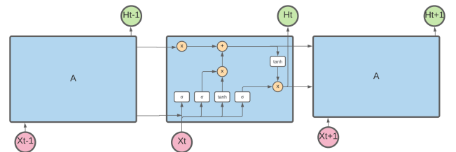
Figure 1. LSTM architecture.
